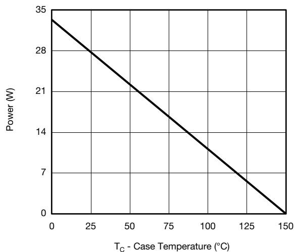
Power, Junction-to-Case
