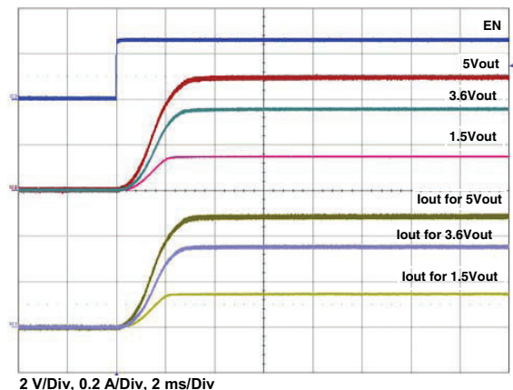
Fig. 26 - Typical Turn-On Delay, Rise Time C_{OUT} = 200 \mu F , C_{IN} = 4.7 \mu F , R_{OUT} = 10 \Omega
