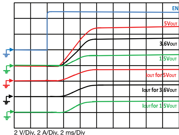
Fig. 19 - Typical Turn-On Delay, Rise Time C_{OUT} = 0.1 \mu F , C_{IN} = 4.7 \mu F , I_{OUT} = 1.5 A
