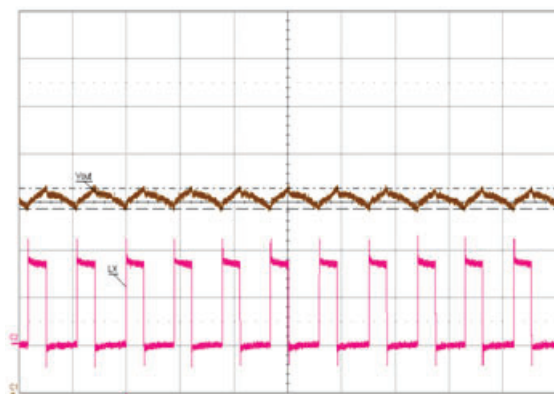
Output Ripple PSM: 3 A Load
