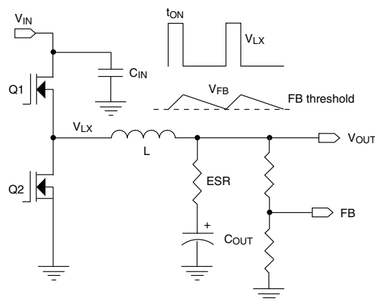
Fig. 1 - PWM Control Method, V_{OUT} Ripple
