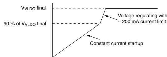
Fig. 9 - LDO Start-Up
