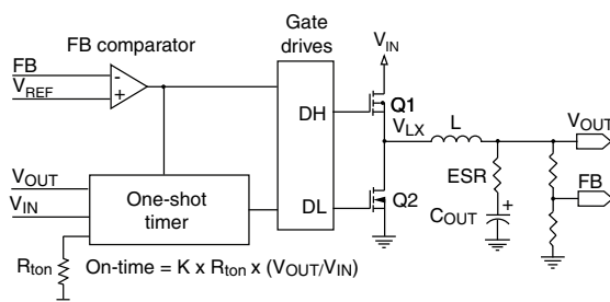
Fig. 2 - On-Time Generation
