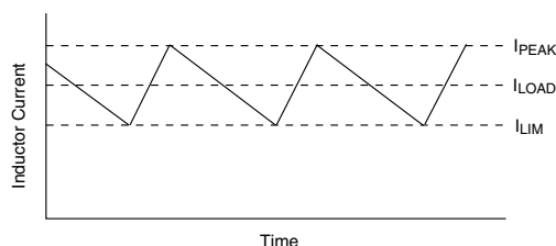
Fig. 8 - Valley Current Limit
