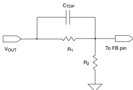
Fig. 12 - Capacitor Coupling to FB Pin
