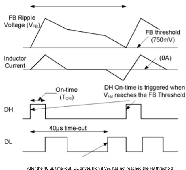
Fig. 5 - Ultrasonic Power-Save Operation
