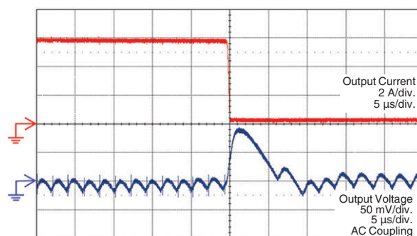
Transient Response in Continuous Conduction Mode (6 A to 0.2 A) (V IN = 12 V, V OUT = 1 V, f SW = 500 kHz)
