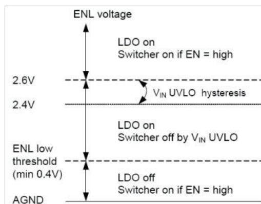
Fig. 11 - ENL Thresholds
