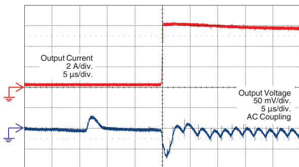
Transient Response in Power Save Mode (0.2 A to 6 A) (V IN = 12 V, V OUT = 1 V, f SW = 500 kHz at 6 A)
