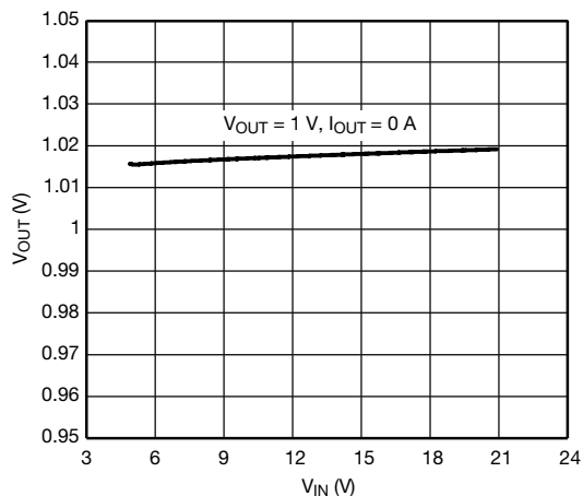
V_{OUT} vs. V_{IN} ( I_{OUT} = 0 A in Power-Save-Mode)
