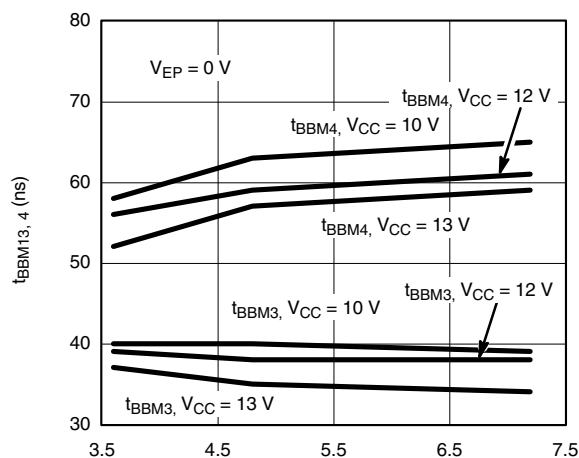
t_{BBM3,4} vs. V_{CC} vs. V_{INDET}
