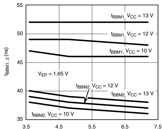
t_{BBM1,2} vs. V_{CC} vs. V_{INDET}
