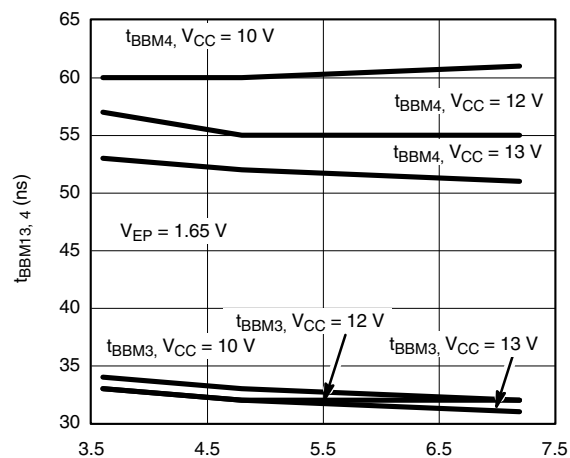
t_{BBM3,4} vs. V_{CC} vs. V_{INDET}
