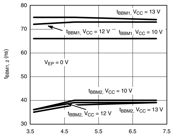
t_{BBM1,2} vs. V_{CC} vs. V_{INDET}
