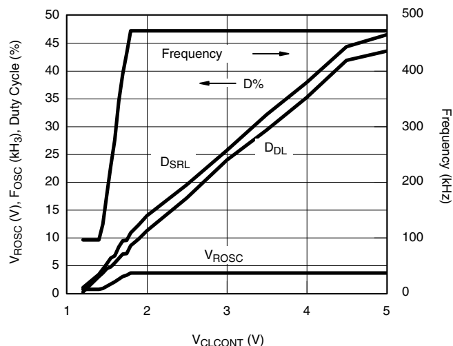
V_{ROSC} , F_{OSC} , and Duty Cycle vs. V_{CLCONT}
