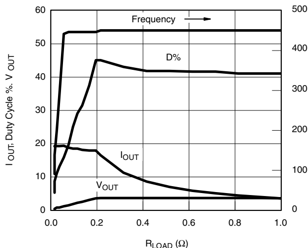
I_{OUT} vs. R_{LOAD} ( V_{IN} = 72 V)
