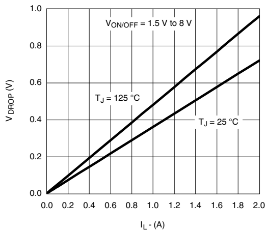
V_{DROP} vs. I_L at V_{IN} = 4.5 V
