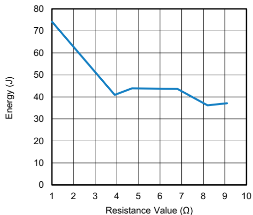
PULSE ENERGY CURVE FOR AC05-CS: 1\ \Omega to 9.1\ \Omega (1.2 / 50 μs; 10 pulses at 30 s interval)
