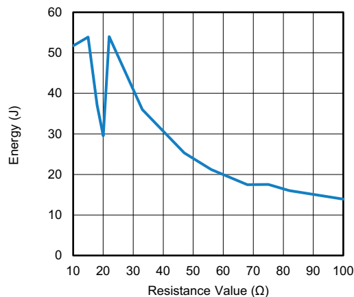
PULSE ENERGY CURVE FOR AC05-CS: 10\ \Omega to 100\ \Omega (1.2 / 50 μs; 10 pulses at 30 s interval)
