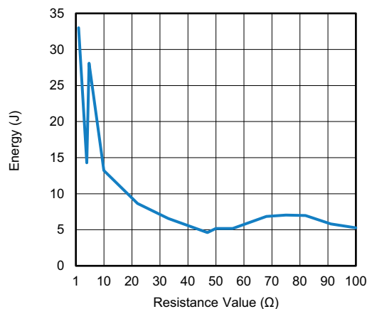
PULSE ENERGY CURVE FOR AC03-CS (1.2 / 50 μs; 10 pulses at 30 s interval)
