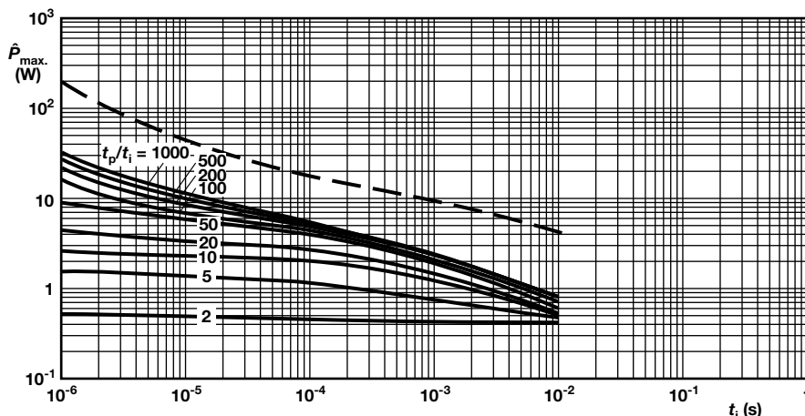
NFR25 Pulse on a regular basis; maximum permissible peak pulse power ( \hat{P}_{\text{max.}} ) as a function of pulse duration ( t_i ), 0.22 \Omega \leq R \leq 1 \text{ k}\Omega
