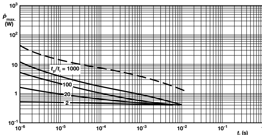
NFR25H Pulse on a regular basis; maximum permissible peak pulse power ( \hat{P}_{\text{max.}} ) as a function of pulse duration ( t_i ), 15 \Omega \leq R \leq 15 \text{ k}\Omega
