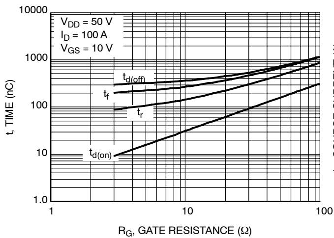
Figure 9. Resistive Switching Time Variation versus Gate Resistance
