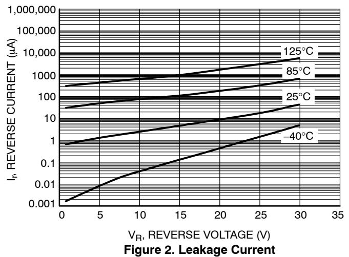
Figure 2. Leakage Current
