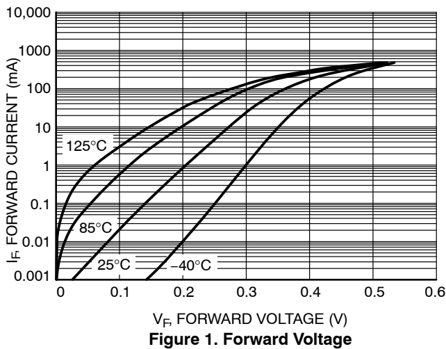
Figure 1. Forward Voltage
