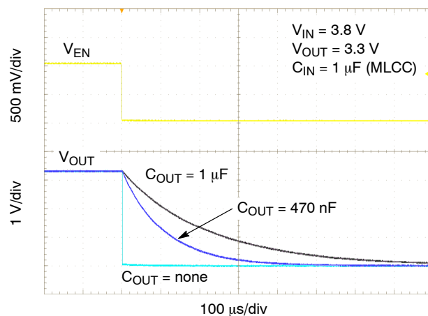
Figure 41. Enable Turn-Off
