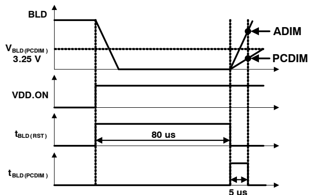
Figure 11. Mode Detection
