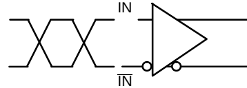
Figure 23. Differential Inputs Driven Differentially
