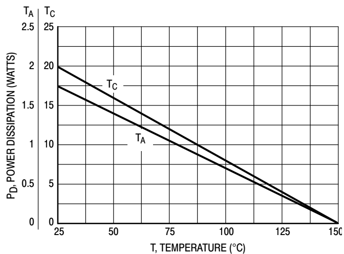
Figure 2. Power Derating
