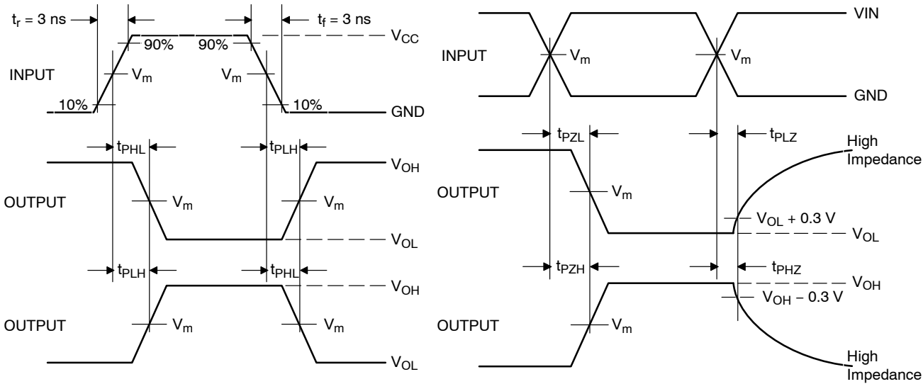
Figure 2. Test Circuit
