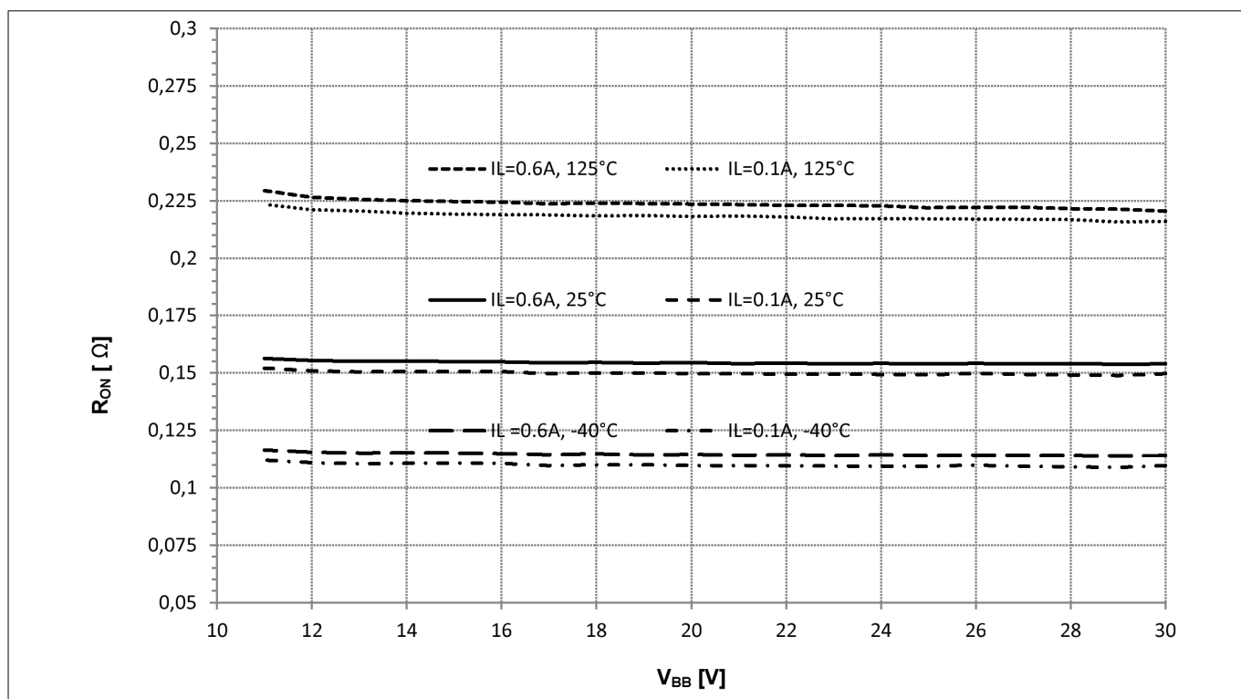
Figure 29 Typ. On-State Resistance ( R_{ON} = f(V_{BB}) , I_L = 0.6 A, I_L = 0.1 A, V_{in} = \text{high} )
