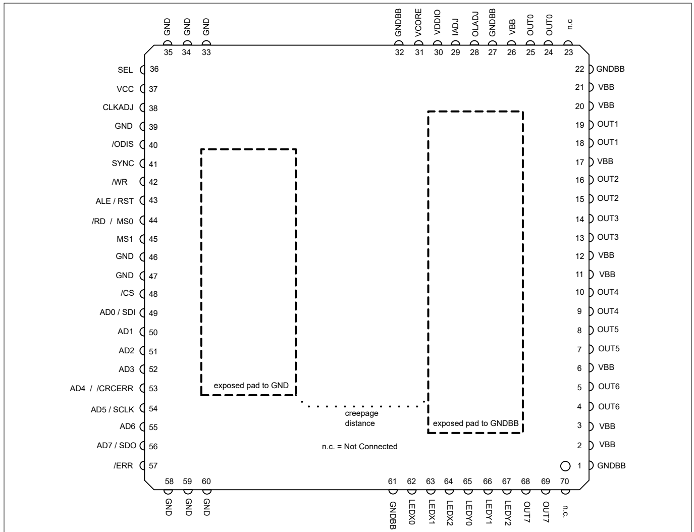
Figure 2 Power PG-VQFN-70 (430 mil)
