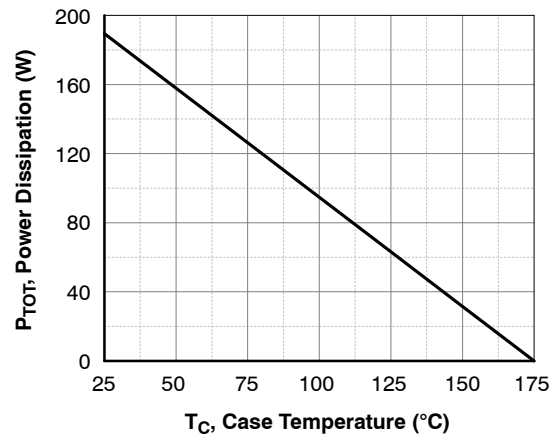
Figure 4. Power Derating
