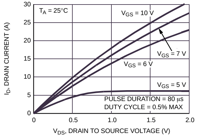
Figure 8. Saturation Characteristics
