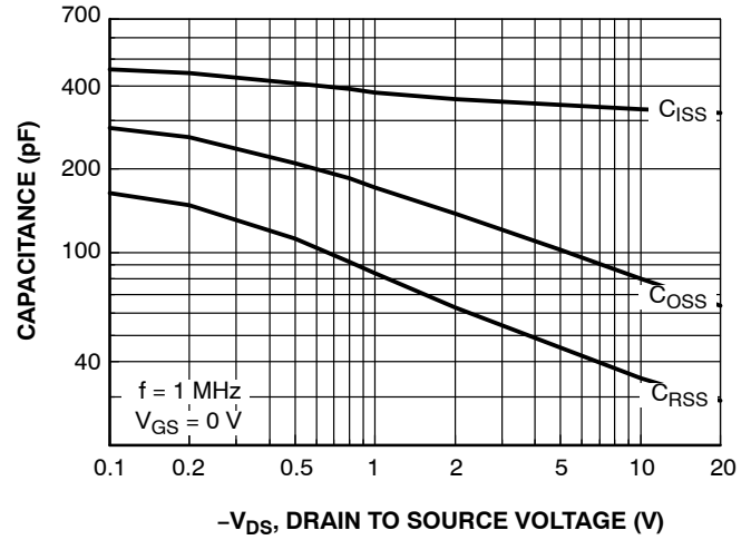
Figure 8. Capacitance Characteristics
