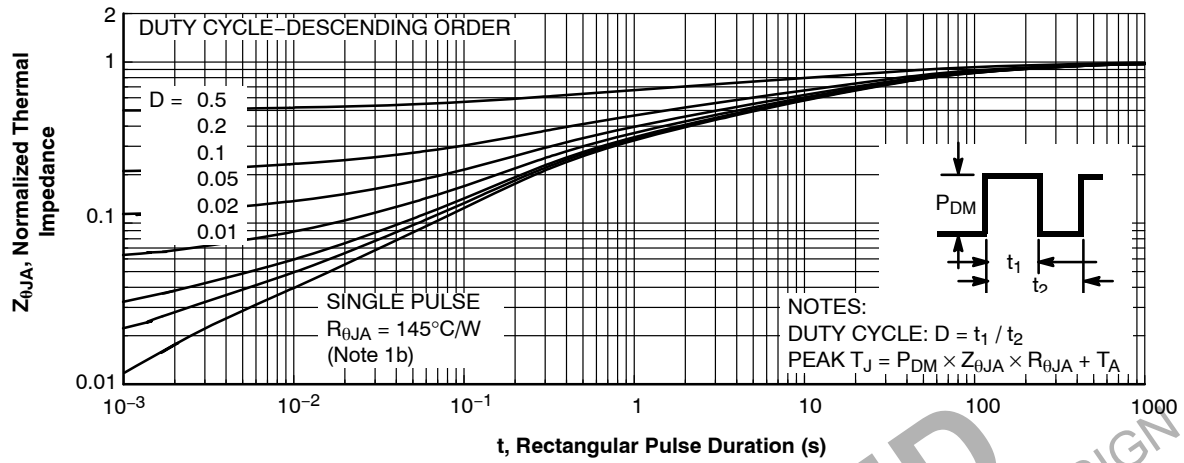
Figure 12. Junction-to-Ambient Transient Thermal Response Curve
