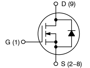
N-CHANNEL MOSFET
