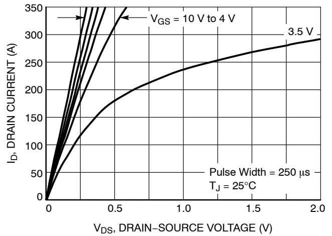
Figure 9. Saturation Characteristics
