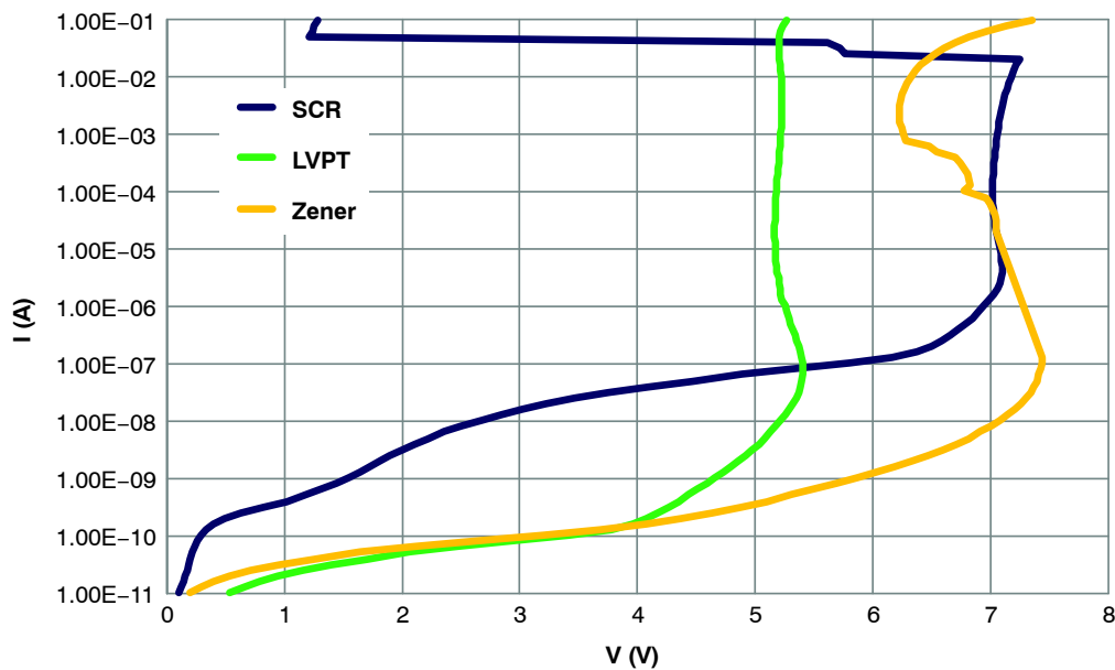
Figure 19. Low Current, DC, IV Characteristic Technology Comparison
