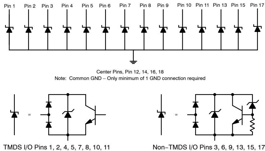
Figure 1. Pin Schematic
