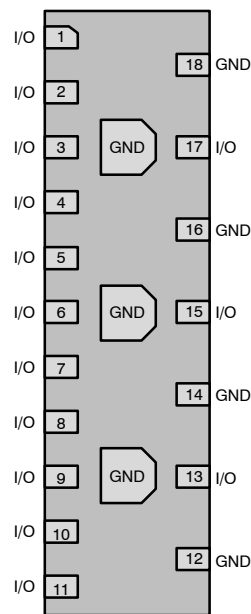
Figure 2. Pin Configuration
