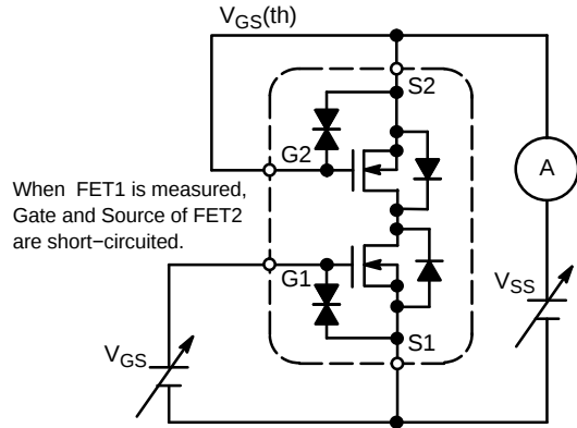
Figure 13. Test Circuit 3
