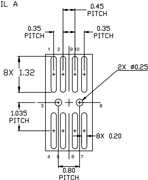
RECOMMENDED MOUNTING FOOTPRINT
