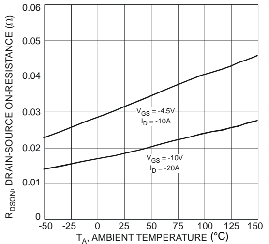
Fig. 18 On-Resistance Variation with Temperature
