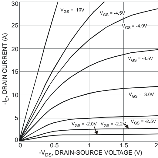
Fig. 13 Typical Output Characteristic
