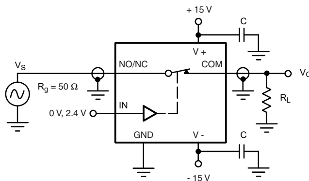
Fig. 4 - Insertion Loss
