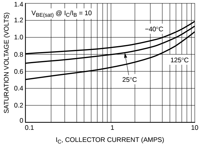
Figure 8. D45VH10 ON-Voltage
