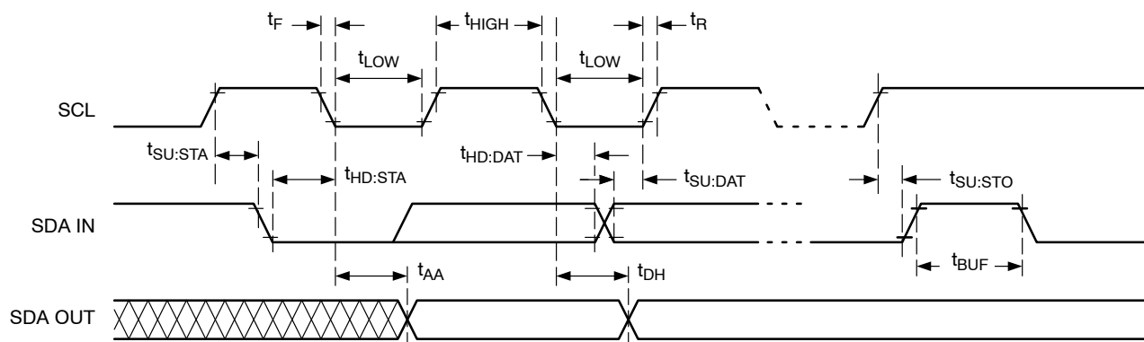
Figure 5. Bus Timing
