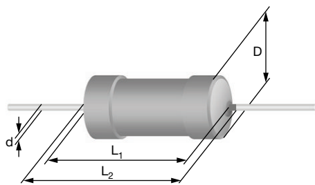
Type with straight leads
