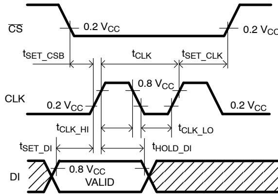
Figure 5. SPI Timing
