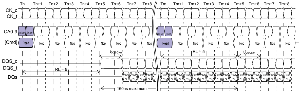
Figure 11: t_{DQCKDS} timing
