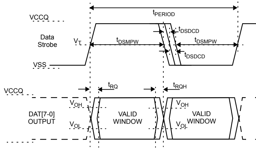
Figure 5. HS400 Device Output Timing
