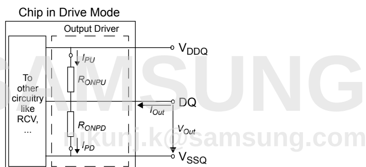
Figure 12. Output Driver: Definition of Voltages and Currents
