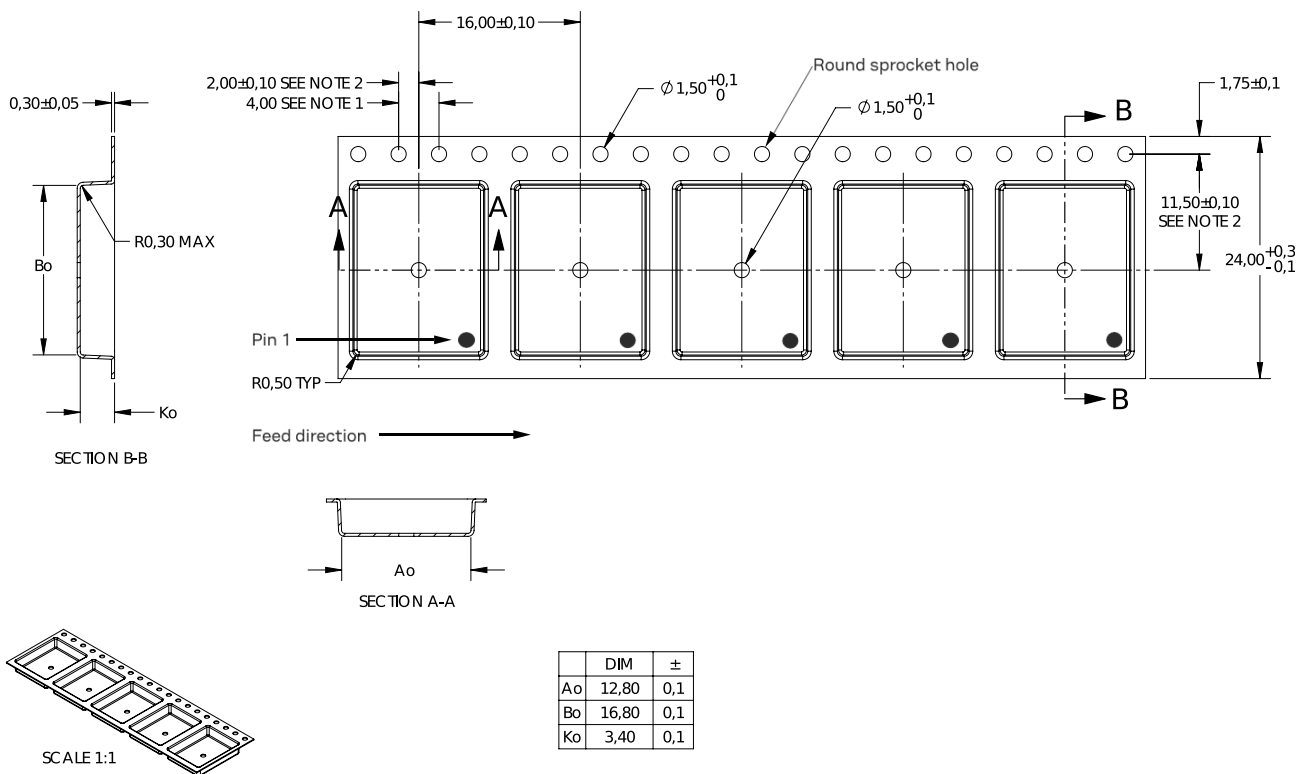
Figure 8: Dimensions (in mm) and orientation for NEO-M8T modules on tape
