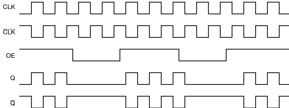
Figure 8. Output Enable (OE) Timing Diagram
