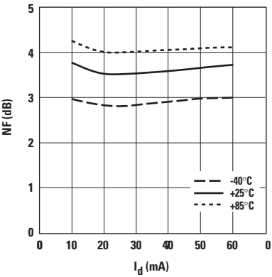
Figure 3. NF vs. I_d and Temperature at 2 GHz.
