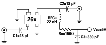
Figure 5. Schematic of 1.9 GHz Circuit.
