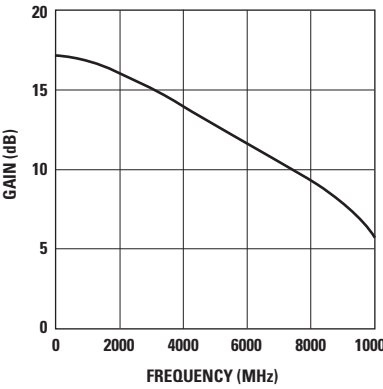
Figure 6. Gain vs. Frequency at I_d = 27 mA.
