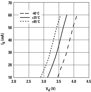
Figure 1. I_d vs. V_d and Temperature.
