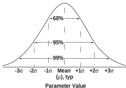
Figure 10. Normal Distribution.
