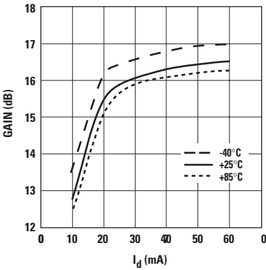
Figure 2. Gain vs. I_d and Temperature at 2 GHz.
