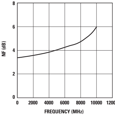
Figure 7. Noise Figure vs. Frequency at I_d = 27 mA.
