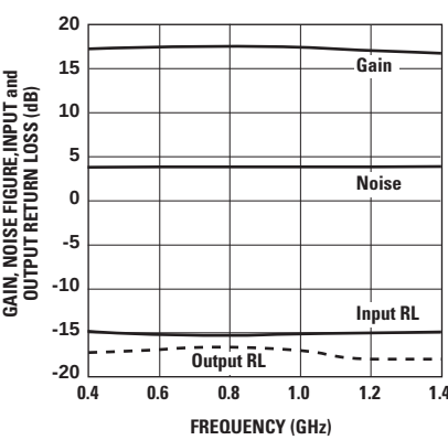
Figure 9. Gain, Noise Figure, Input and Output Return Loss Results.
