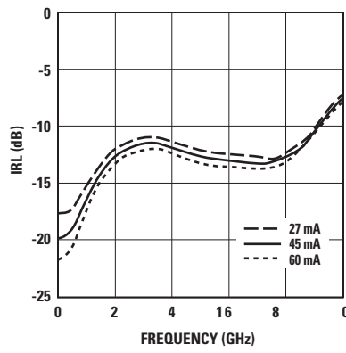
Figure 14. Input Return Loss vs. Frequency and I_d .
