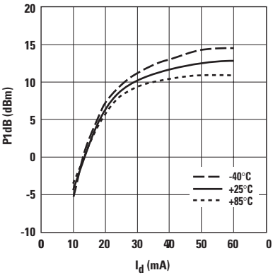
Figure 4. P1dB vs. I_d and Temperature at 2 GHz.
