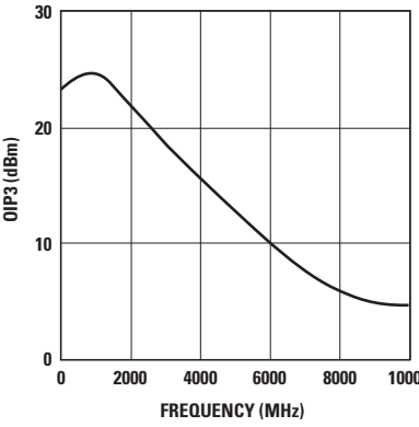
Figure 9. OIP3 vs. Frequency at I_d = 27 mA.
