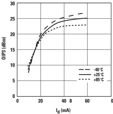
Figure 5. OIP3 vs. I_d and Temperature at 2 GHz.
