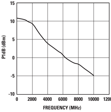
Figure 8. P1dB vs. Frequency at I_d = 27 mA.
