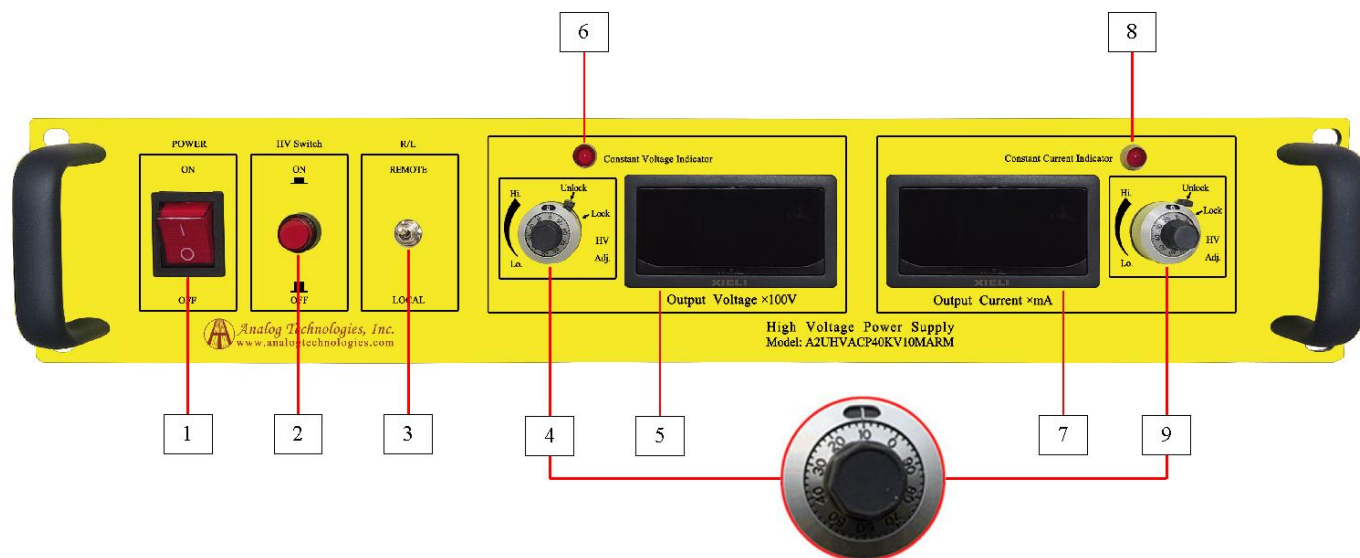
Figure 2. Front Panel
