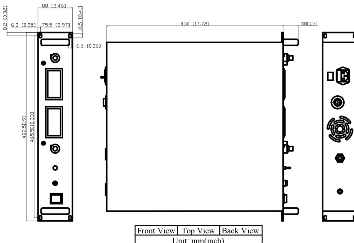
Figure 7. Dimensions for A2UHVACP40KV10MARM
