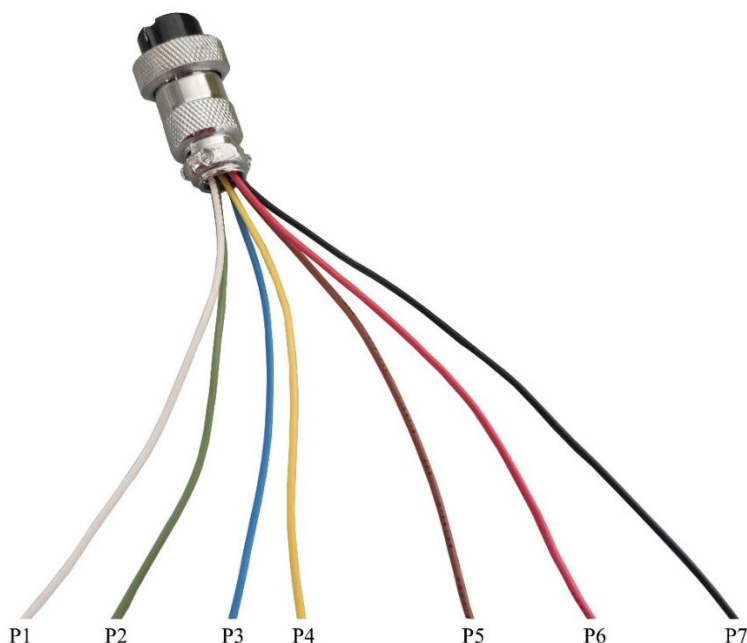
Figure 4. 8-pin Connector
