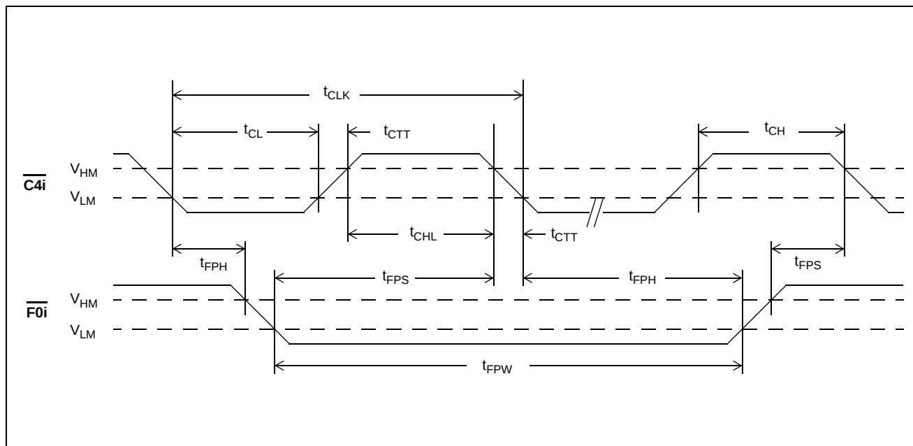
Figure 10 - Clock Timing
