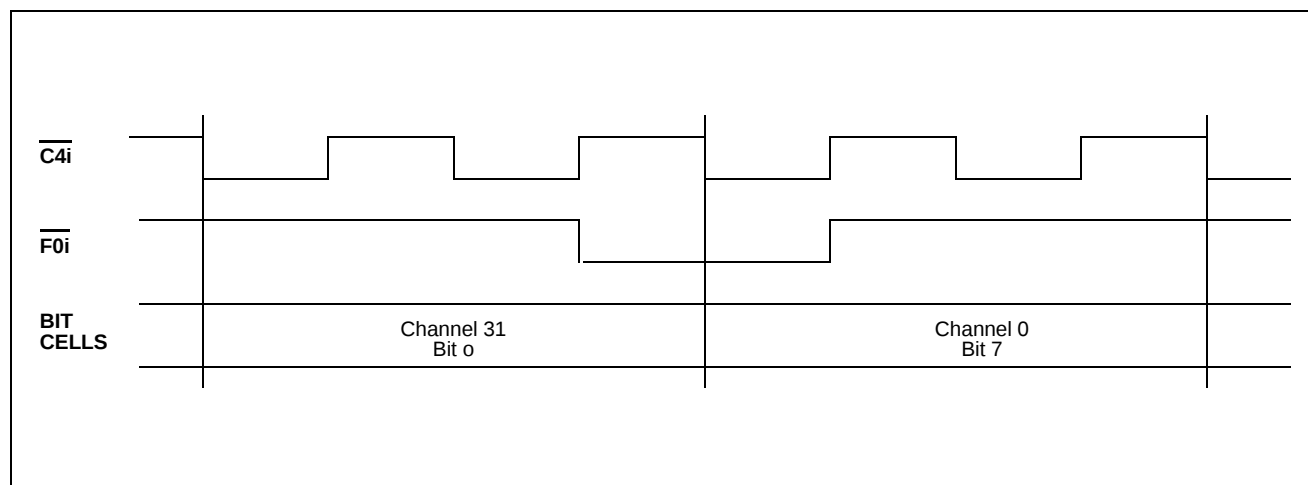
Figure 9 - Frame Alignment
