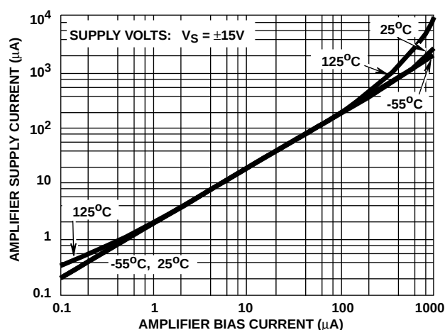
FIGURE 19. AMPLIFIER SUPPLY CURRENT vs AMPLIFIER BIAS CURRENT
