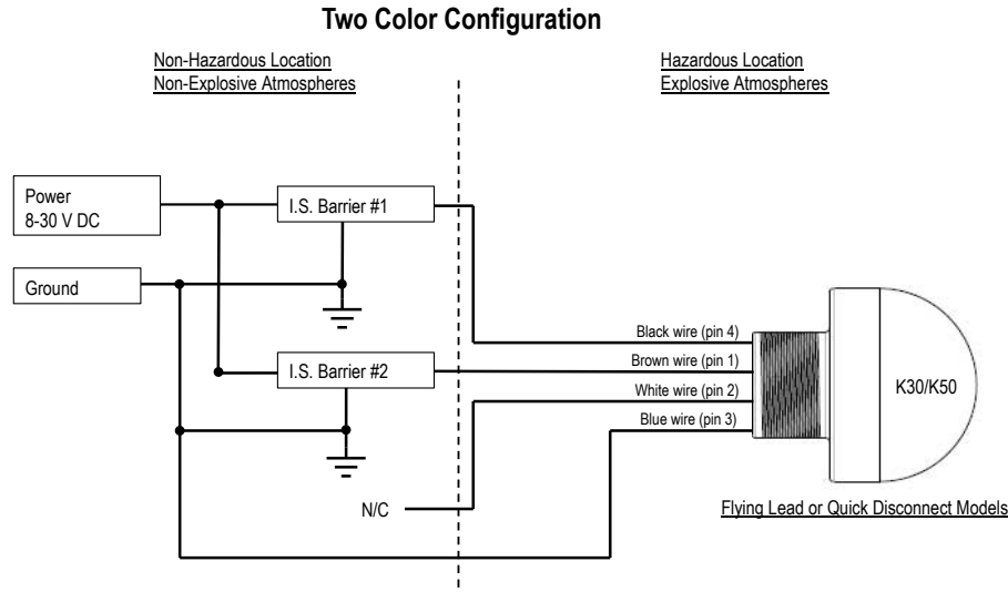
Figure 2. Control Drawing 2-Color Configuration
