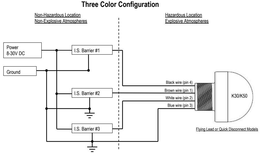
Figure 3. Control Drawing 3-Color Configuration
