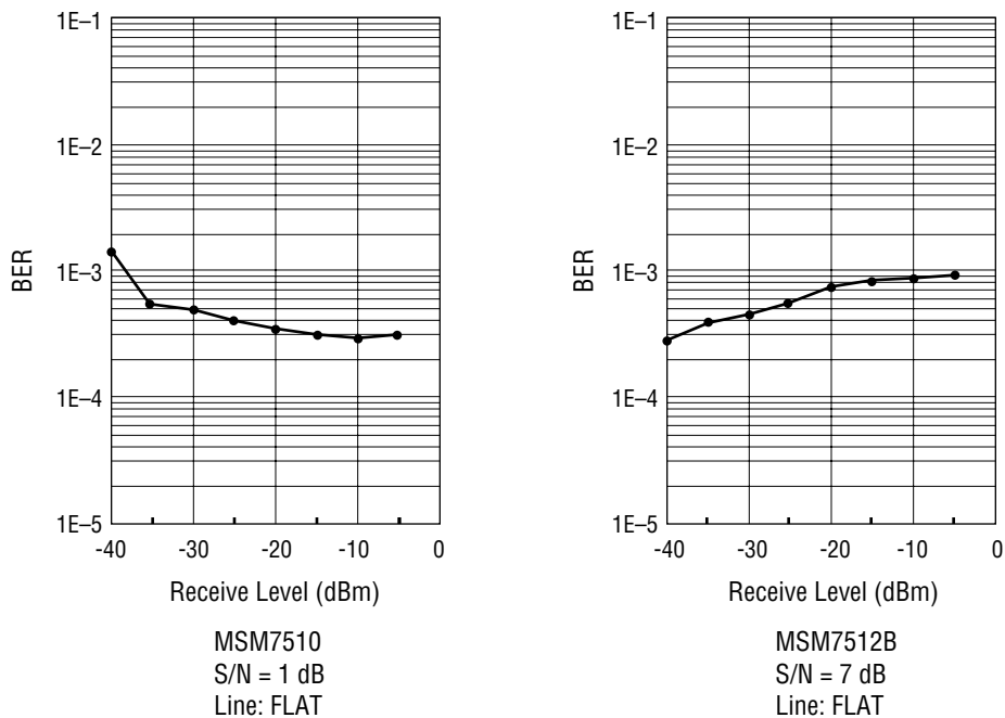
Figure 6-4 MSM7510/7512B Receive Level vs. BER
