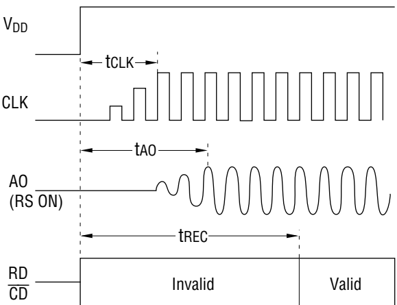
Figure 8-1 Response Time when Power is Turned On
