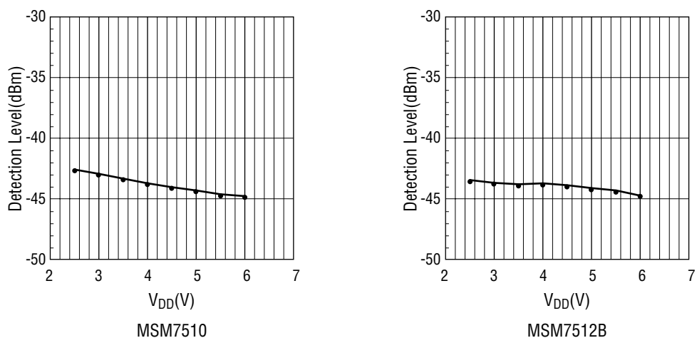
Figure 10-3 Power Voltage Dependency for Carrier Detection (CD ON) Levels
