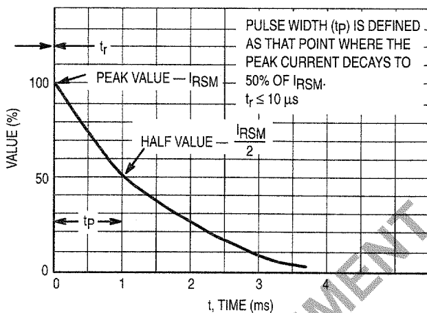
Figure 5. Pulse Waveform
