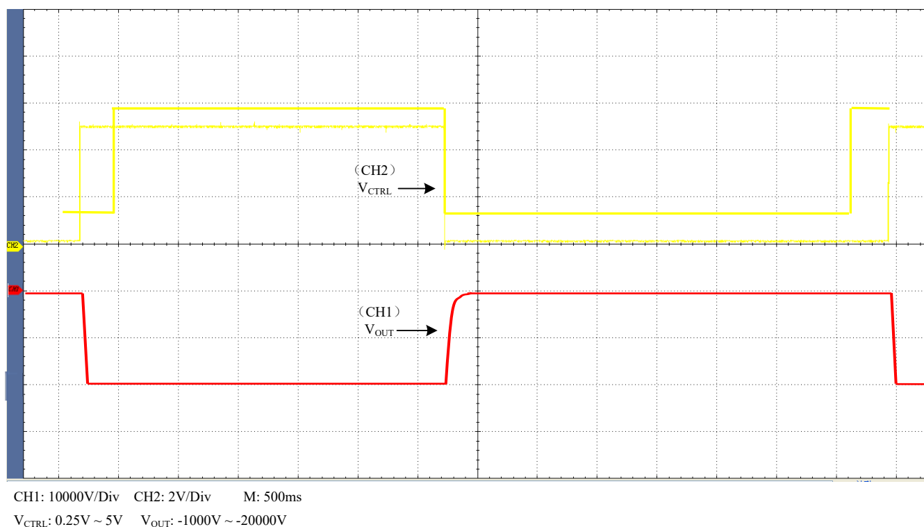
Figure 5. Square Wave
