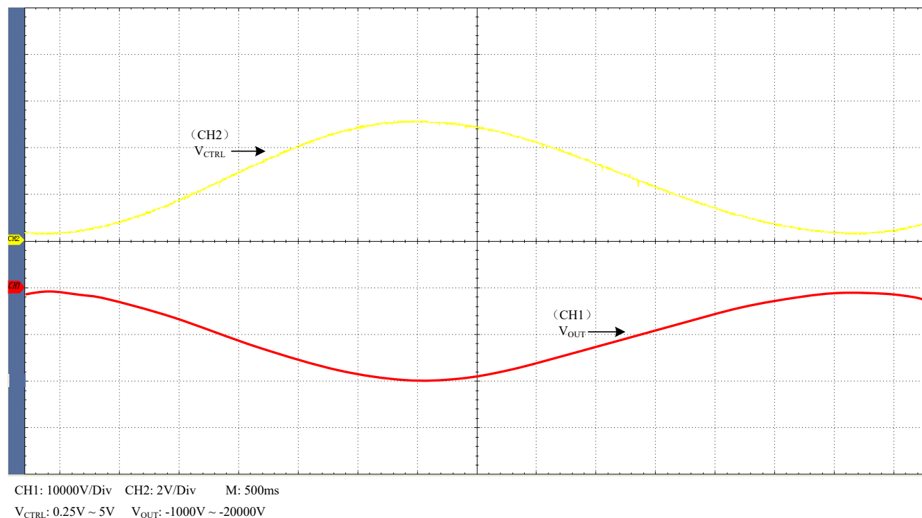
Figure 4. Sine Wave
