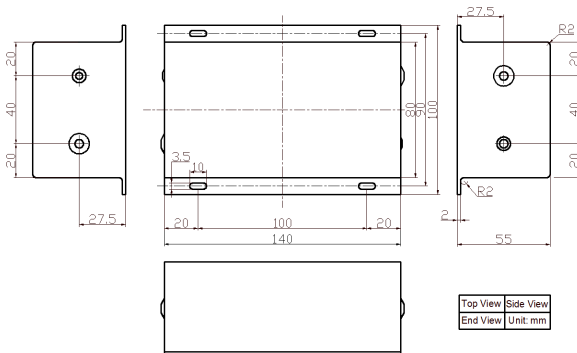
Figure 11. Dimensions for AHV24VN20KV1MAW
