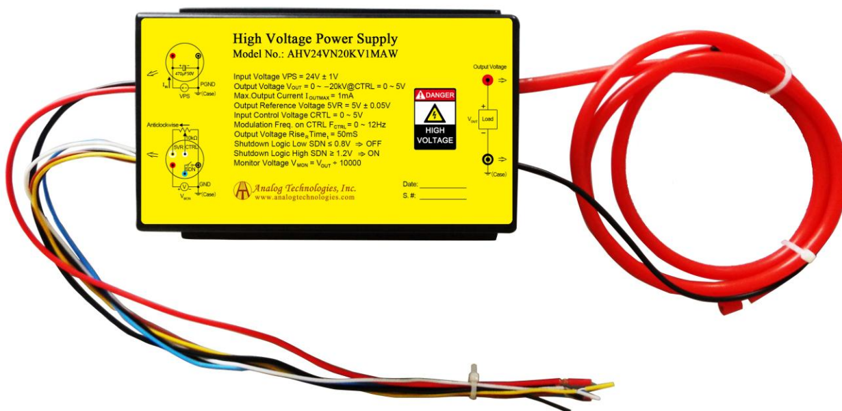
Figure 10. Leads of AHV24VN20KV1MAW
