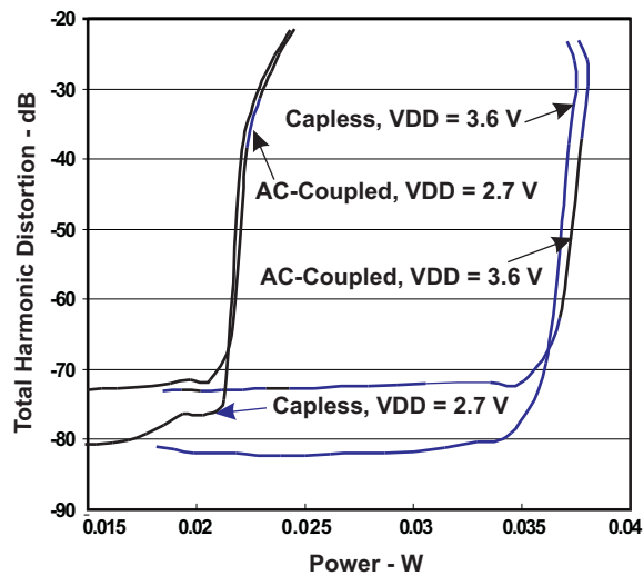
Figure 5. Headphone Power vs THD, 16 \Omega Load
