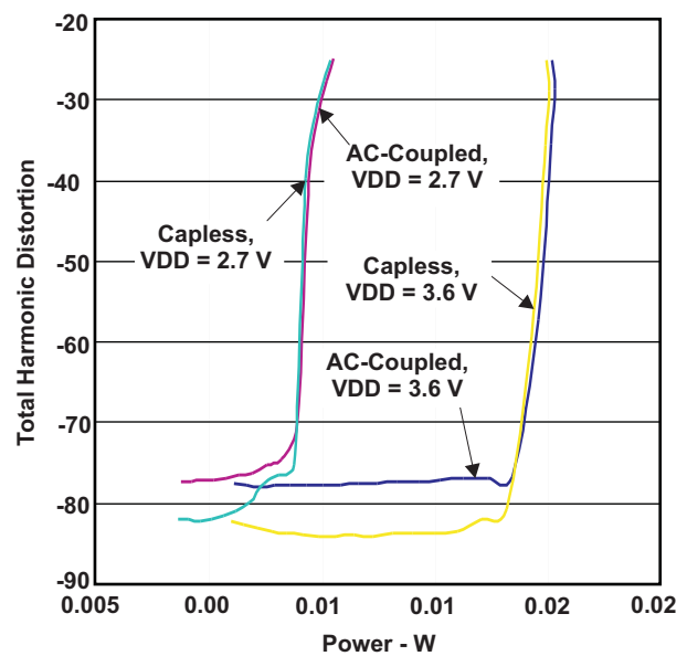
Figure 6. Headphone Power vs THD, 32 \Omega Load
