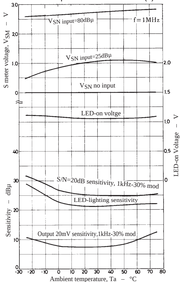
AM Temperature Characteristic(2)
