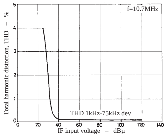
Distortion Characteristic
