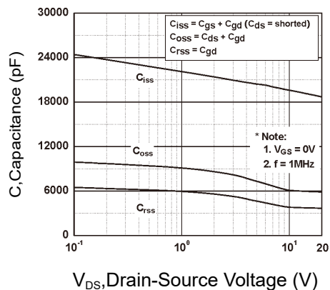
Figure 5: Capacitance Characteristics
