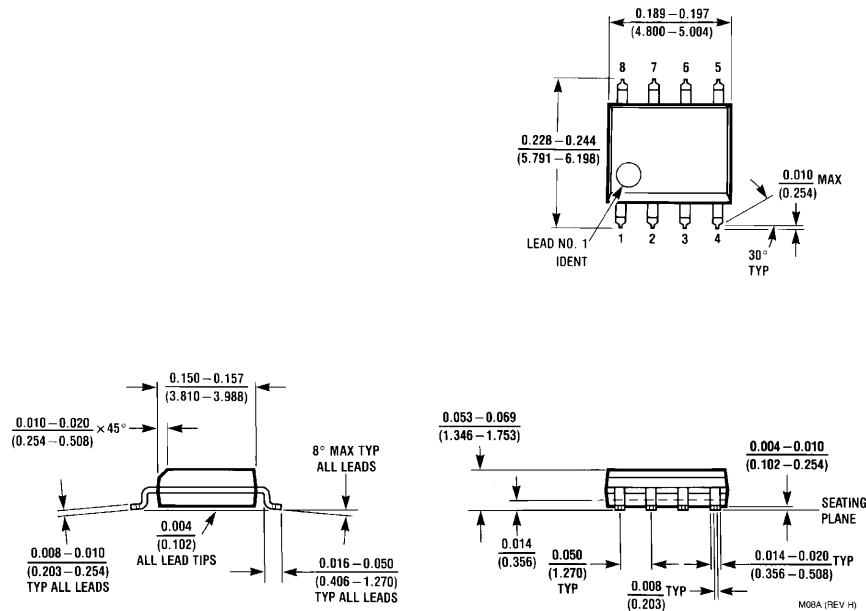
Small Outline (SO-8) Package (M) Order Number LM285M-2.5, LM285AM-2.5, LM285AXM-2.5, LM285AYM-2.5, LM285BXM-2.5, LM285BYM-2.5, LM385M-2.5, LM385AM-2.5, LM385AXM-2.5, LM385AYM-2.5, LM385BM-2.5, LM385BXM-2.5 or LM385BYM-2.5 NS Package Number M08A
