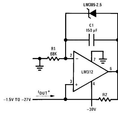
Precision 1 µA to 1 mA Current Sources
