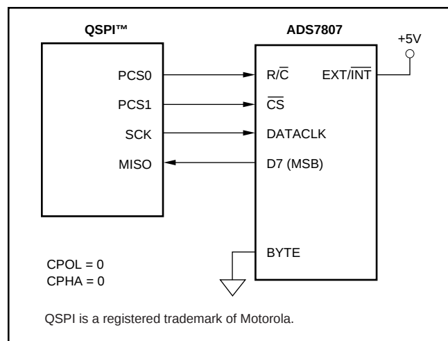
FIGURE 15. QSPI Interface to the ADS7807. Processor Initiates Conversions.
