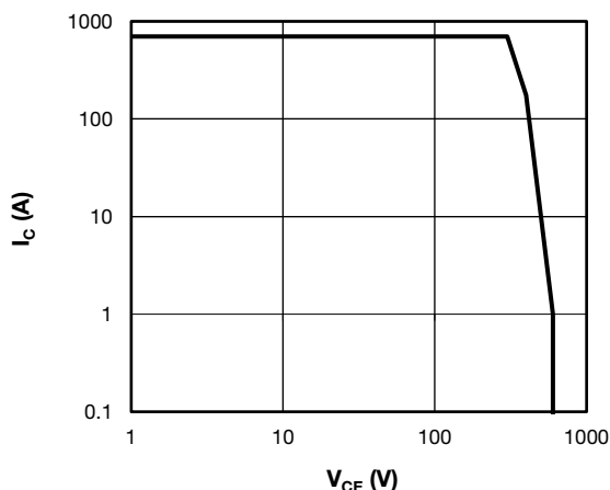
Fig. 17 - Trench IGBT Reverse BIAS SOA T_J = 175^\circ\text{C} , I_C = 700\text{ A} , R_g = 1.5\ \Omega , V_{GE} = +15\text{ V}/0\text{ V} , V_{CC} = 300\text{ V} , V_p = 600\text{ V}
