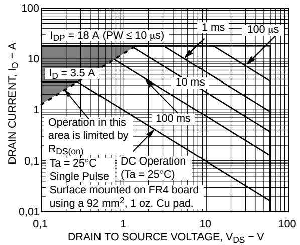
Figure 11. SOA
