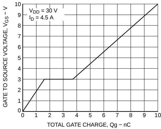
Figure 10. V_{GS} - Q_g
