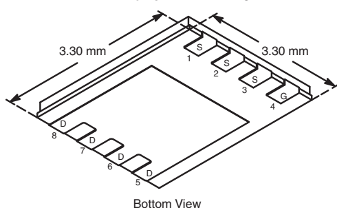
PowerPAK® 1212-8
