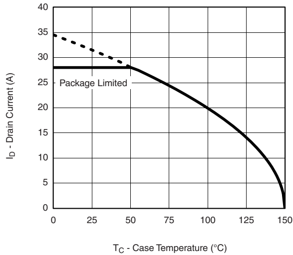
Current Derating*
